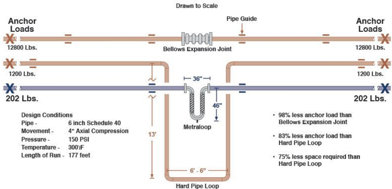
Metraloop vs Bellows vs Hard Pipe Loop Comparison
