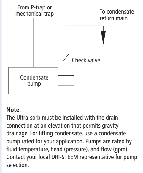
Figure 29-3: Lifting condensate (Models LV and LH)
