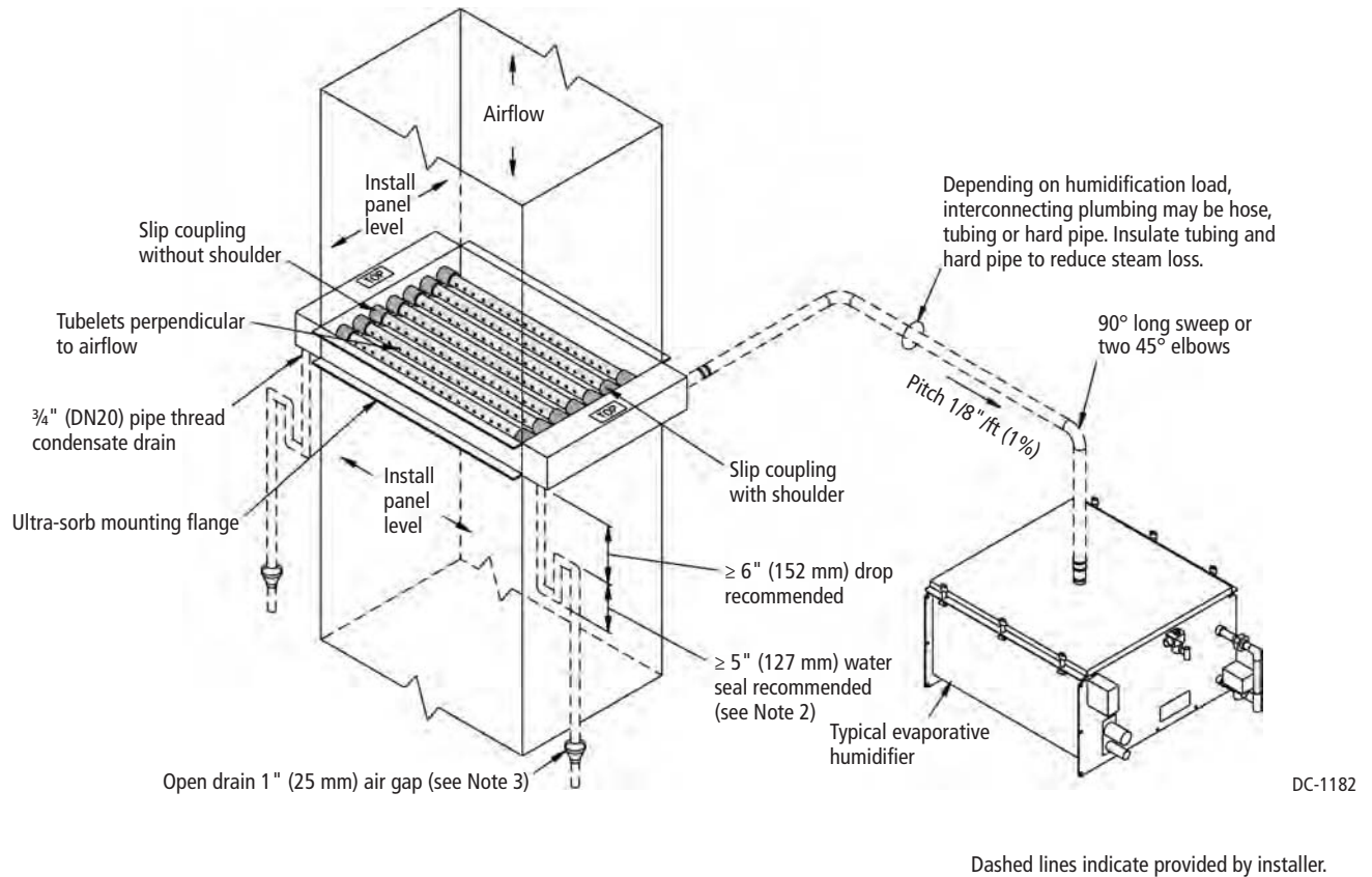
Figure 25-1: Ultra-sorb Model LH in a vertical airflow (evaporative steam application shown)
