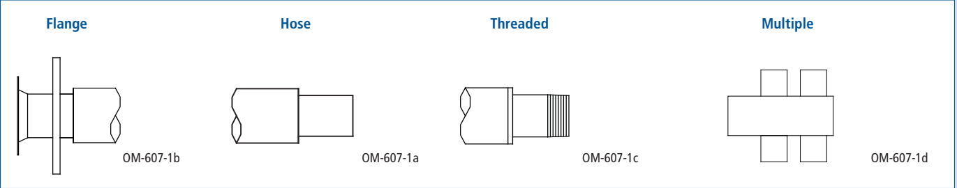
Figure 13-1: Ultra-sorb Models LV and LH steam inlet types
