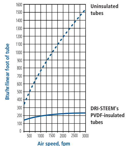
Figure 7-1: Dispersion tube heat loss vs. airspeed at 50 °F (10 °C) for a 3" (76 mm) o.c. tube bank, 1½" (DN40) dia. stainless steel tubes with 212 °F (100 °C) internal wall temperature
