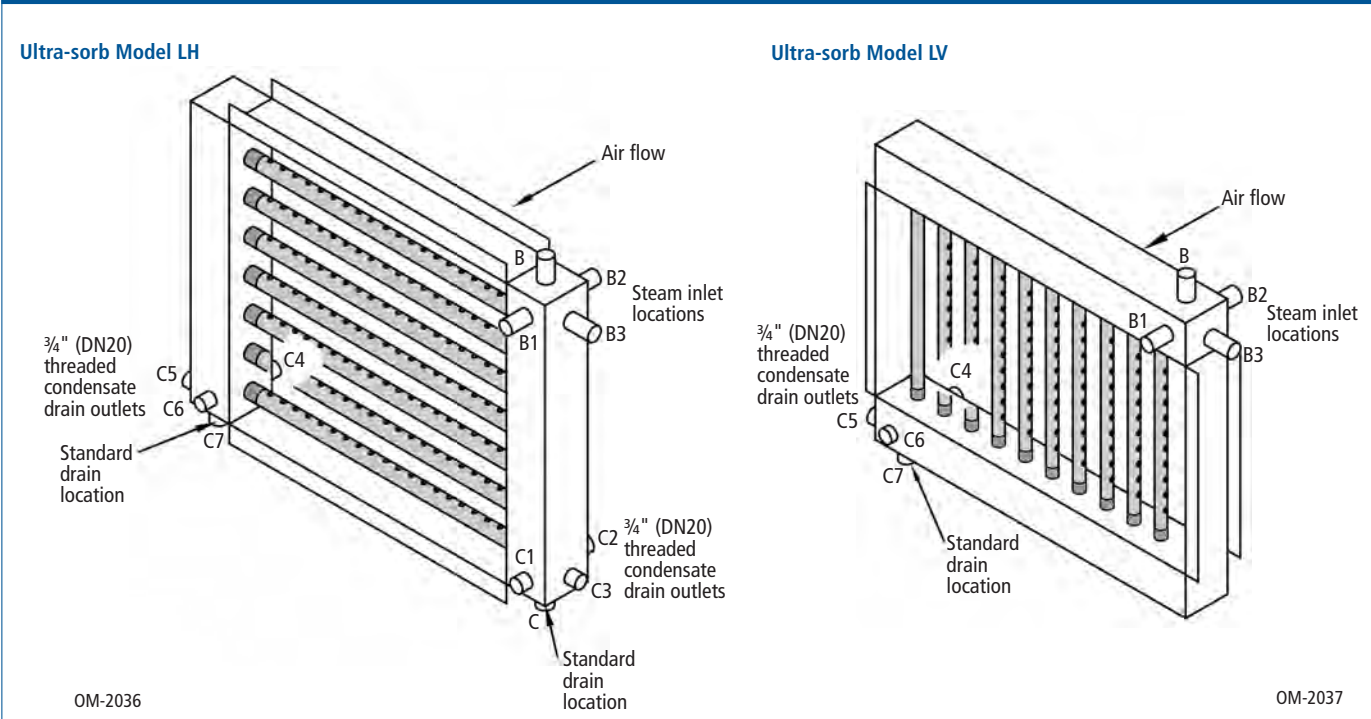
Figure 13-2: Ultra-sorb Models LV and LH steam inlet and condensate outlet positions
