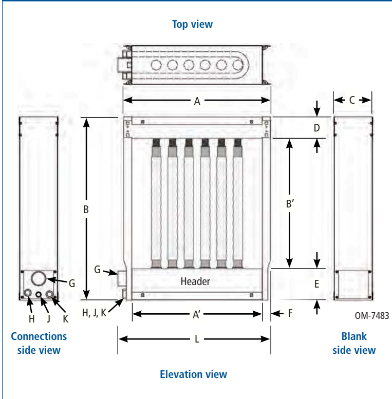
Figure 11-1: Ultra-sorb Model XV dimensions
