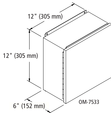
Figure 21-2: Control cabinet for Ultra-sorb Model XV solenoid valve and temperature switch
