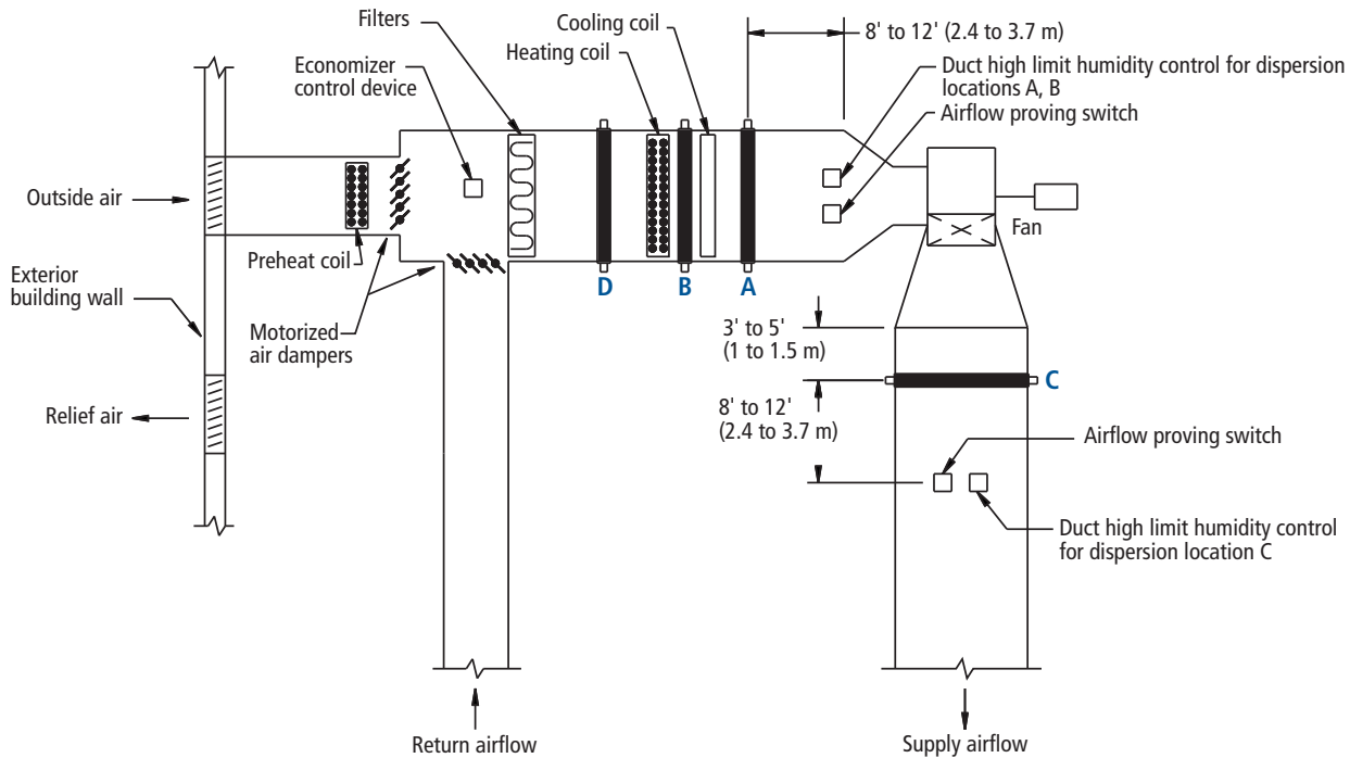
Figure 20-1: Placing a dispersion assembly in an air handling unit
