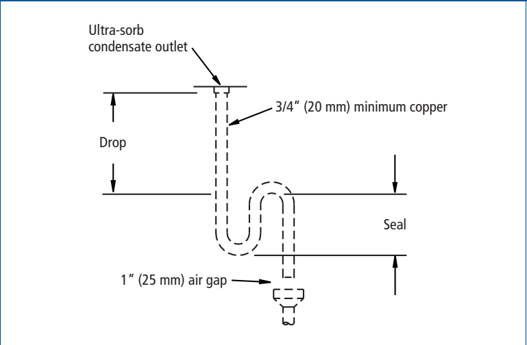
Figure 29-2: P-trap water seal dimensions (Models LV and LH)
