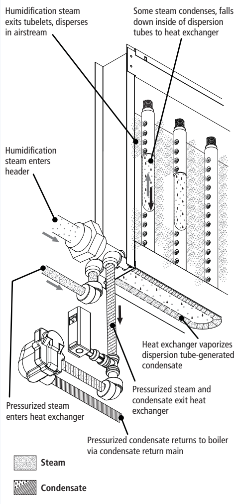
Figure 4-2: Ultra-sorb Model XV simultaneously vaporizes generated condensate and returns pressurized condensate
