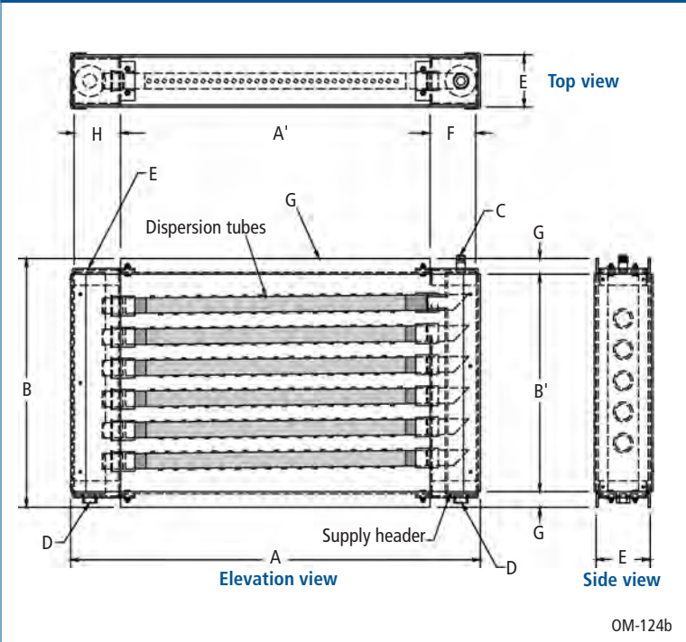
Figure 15-1: Ultra-sorb Model LH dimensions
