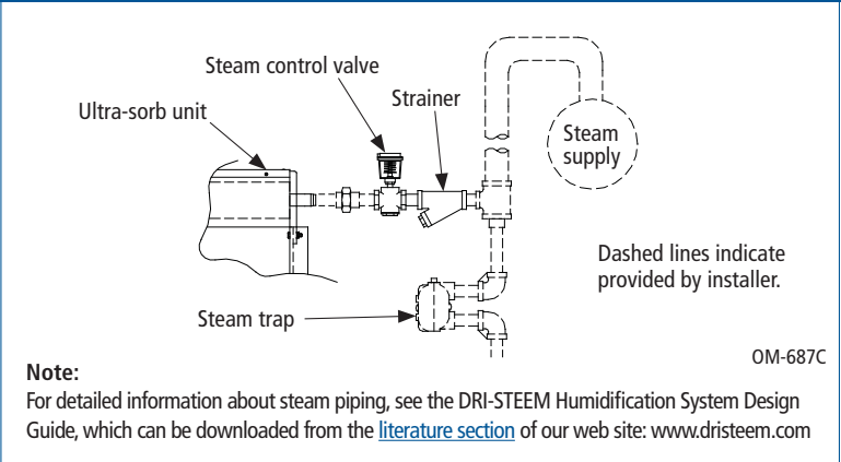
Figure 29-1: Connection to a boiler (pressurized steam applications)
