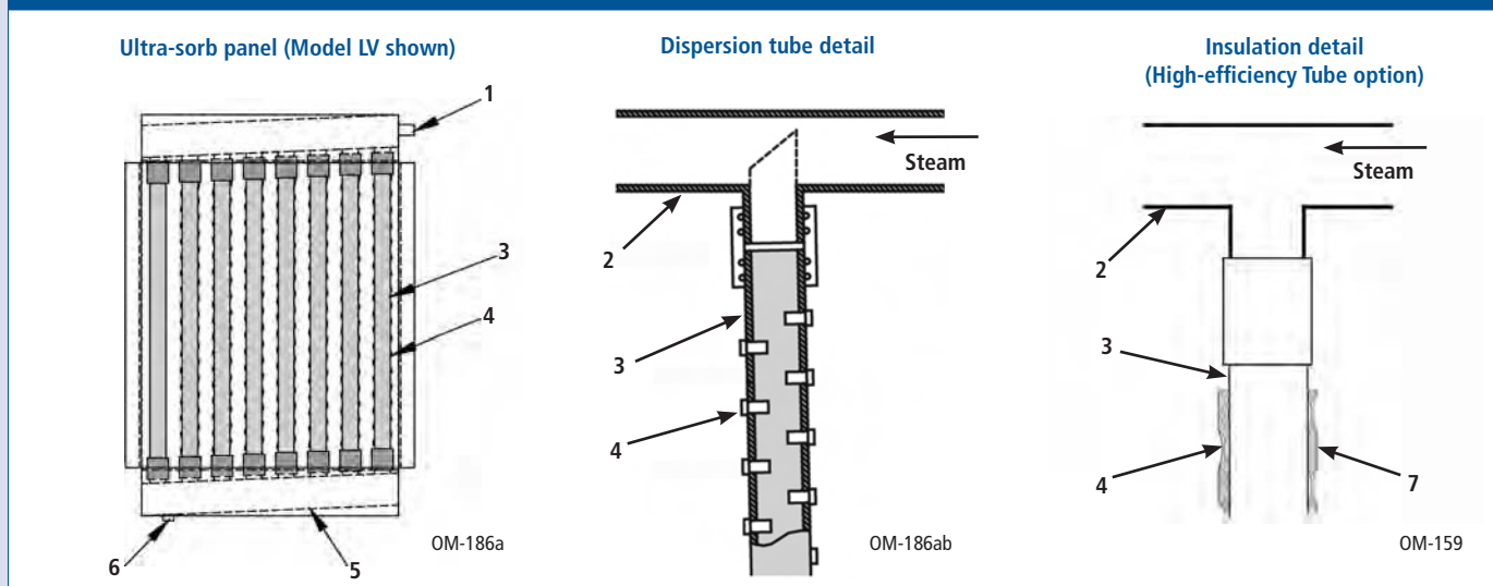
Figure 12-1: Ultra-sorb Models LV and LH components
