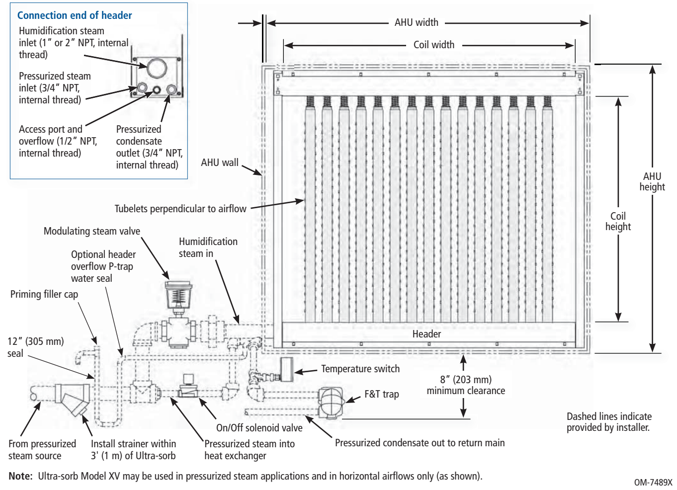
Figure 22-1: Ultra-sorb Model XV in an air handler
