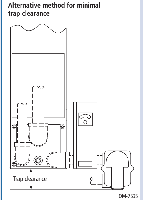
Figure 21-3: Ultra-sorb Model XV piping components
