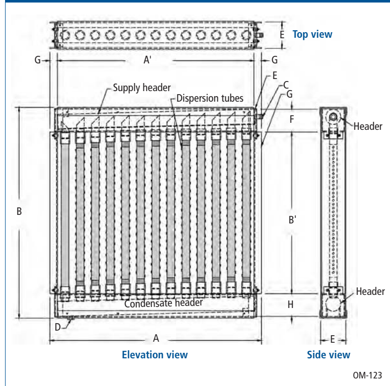
Figure 14-1: Ultra-sorb Model LV dimensions
