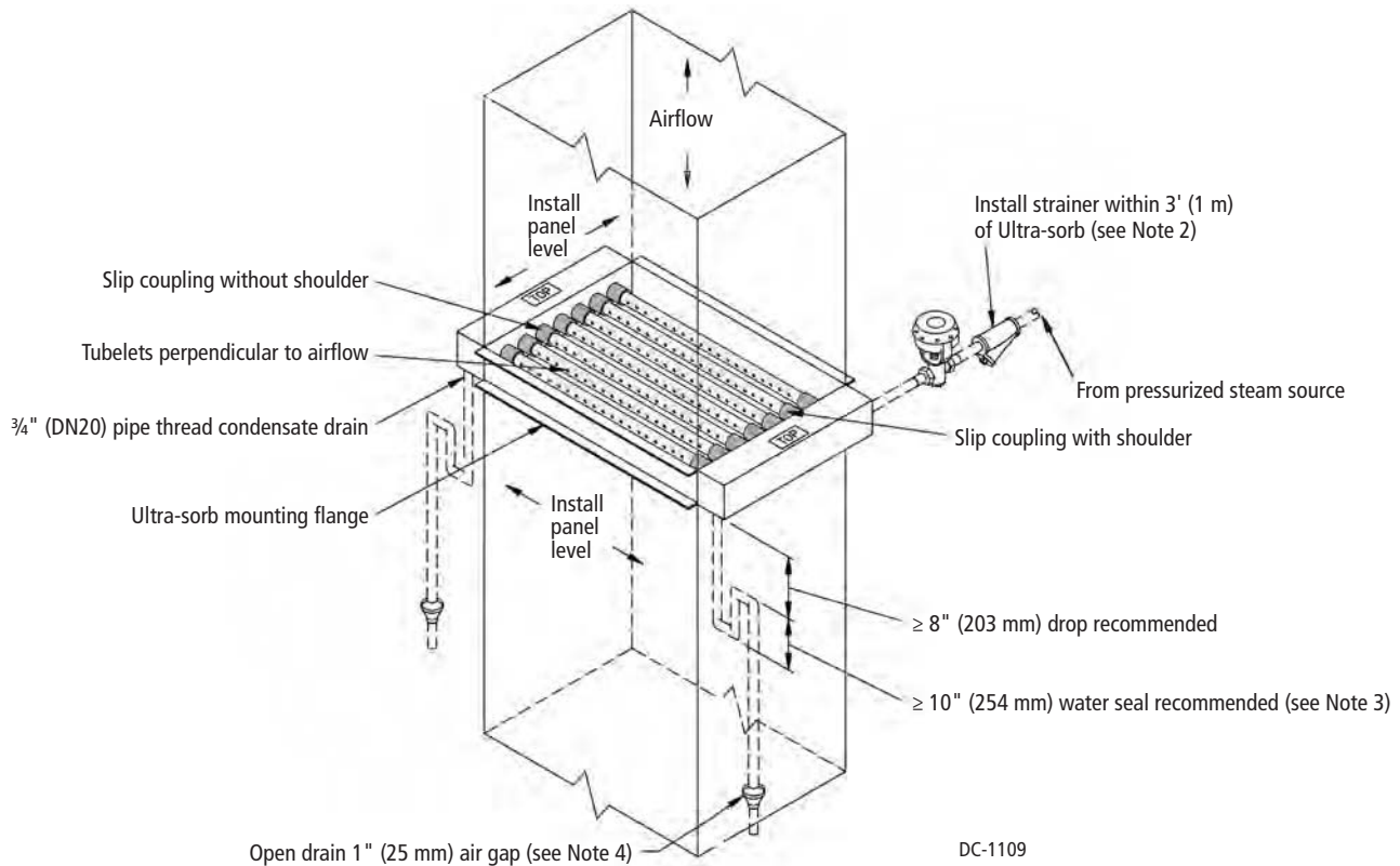
Figure 26-1: Ultra-sorb Model LH in a vertical airflow (pressurized steam application shown)
