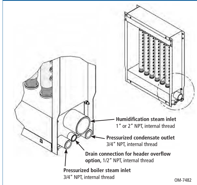
Figure 10-1: Ultra-sorb Model XV connections
