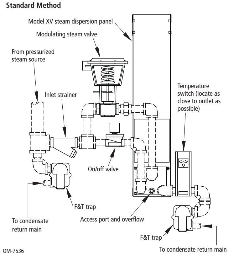
Figure 21-1: Ultra-sorb Model XV piping components
