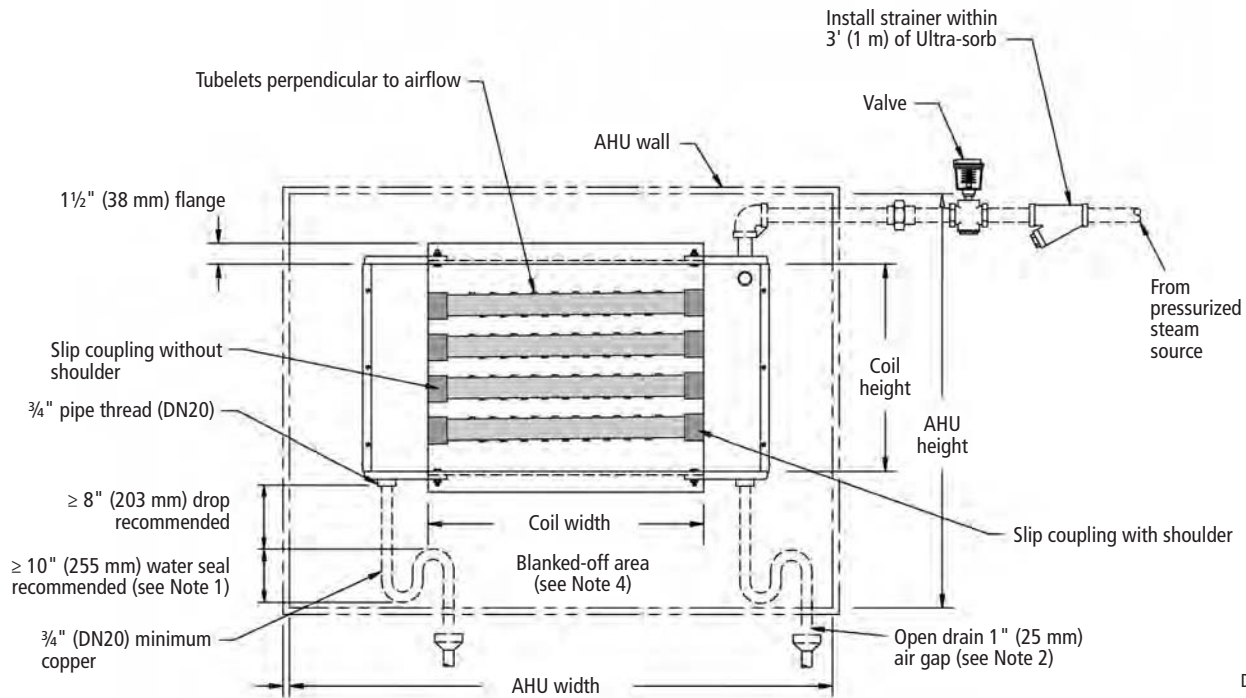
Figure 24-1: Mounting Ultra-sorb Model LH in a horizontal airflow (pressurized steam applications only)
