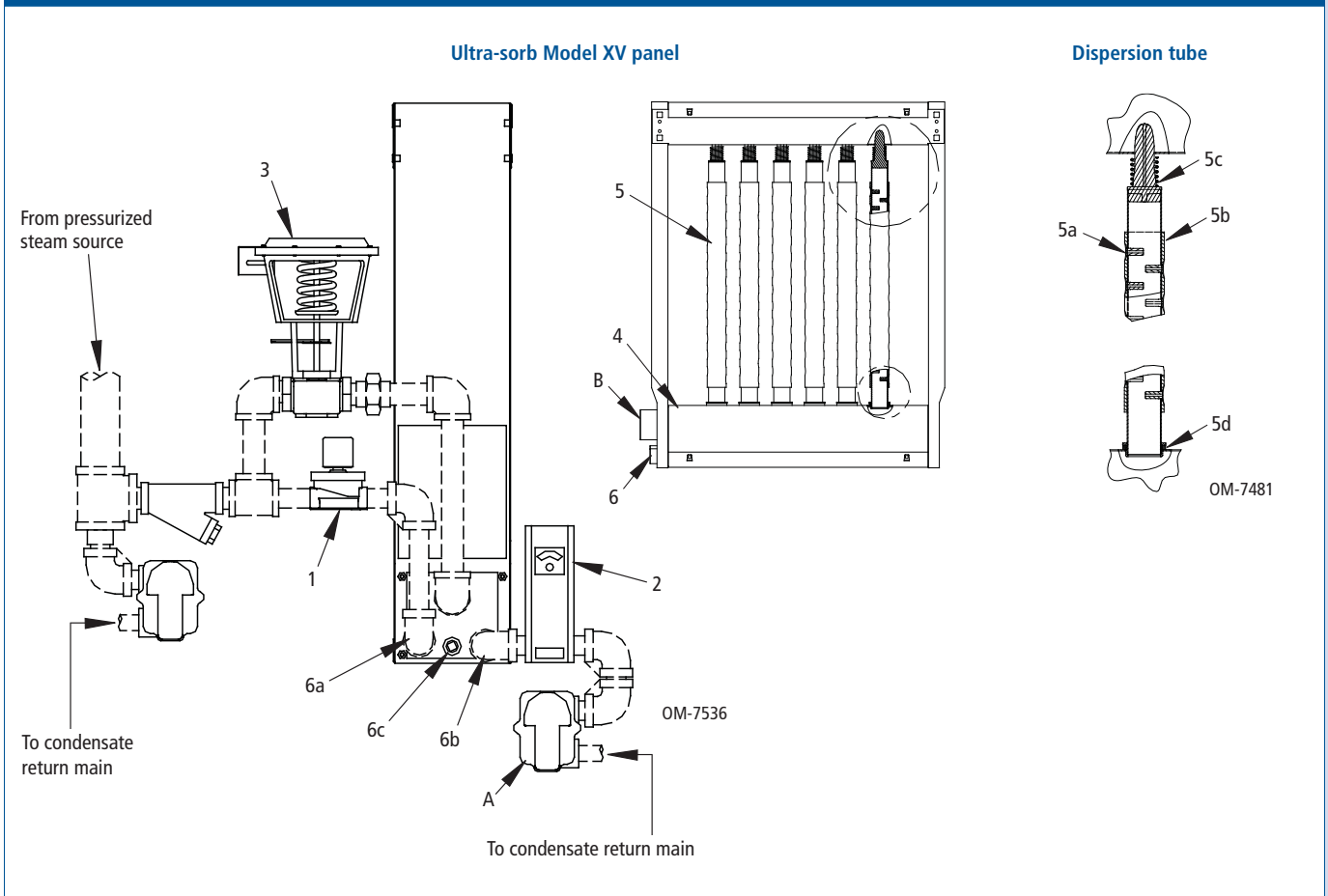
Figure 9-1: Ultra-sorb Model XV components
