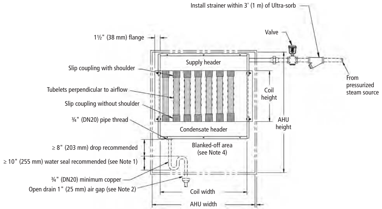
Figure 23-1: Mounting Ultra-sorb Model LV in a horizontal airflow (pressurized steam application shown)
