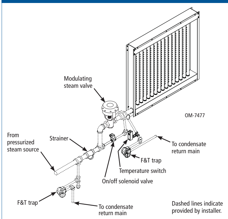
Figure 27-1: Ultra-sorb Model XV piping
