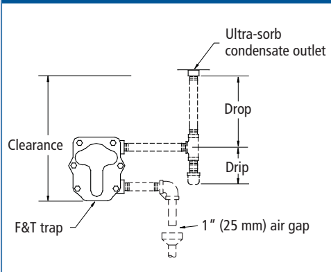
Figure 28-1: F&T trap dimensions (Models LV and LH)
